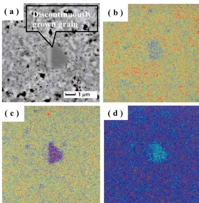
Figure 6 (a) The reflection electron image of the polished surface of the 5% glass added-specimen sintered at 1000°C for 10 h in the sealed platinum container. Distribution of (b) Ba, (c) Co and (d) Fe on the same surface of the sintered specimen. The contrast of (b), (c) and (d) means that the brighter part is richer in the element.
