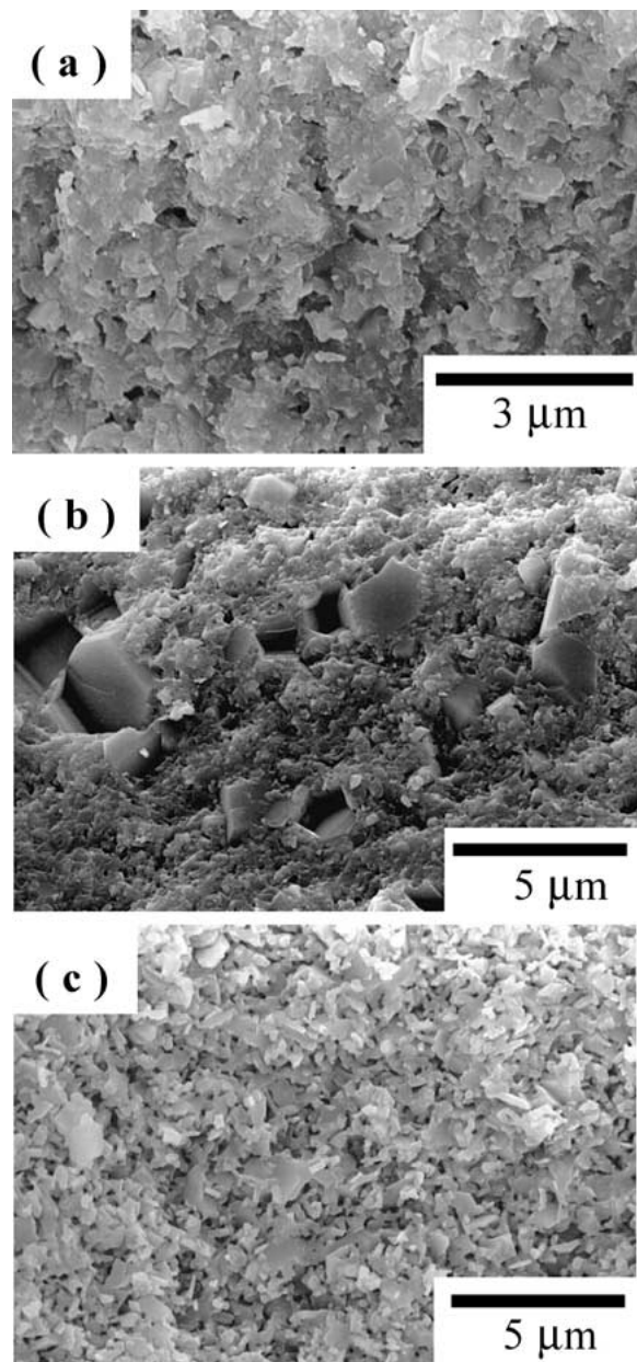
Figure 5 SEM photographs of fractured surfaces of the 5% glass added-specimen sintered at 1000°C (a) for 1 h in air, (b) for 10 h in the sealed platinum container and (c) the 0% glass added-specimen sintered at 1000°C for 10 h in the sealed platinum container.
