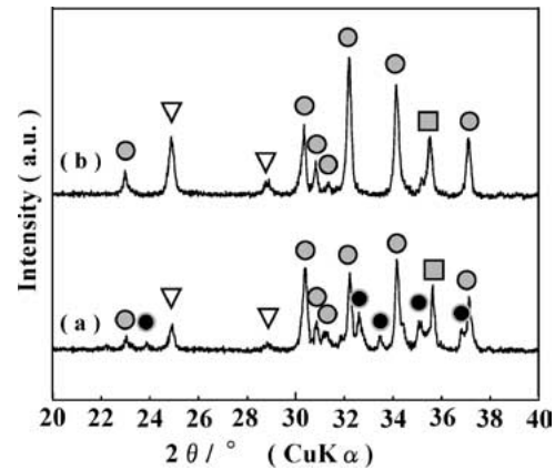
Figure 7 XRD patterns of the 0% glass added-specimen sintered at 1000^\circ\text{C} for 10 h together with (a) the additive glass powder pellet and (b) \text{MgF}_2 powder pellet in the sealed platinum container. (●): \text{Co}_2\text{Z} , (○): Ba-M, (▽): \text{BaF}_2 (□): Spinel ferrite.
