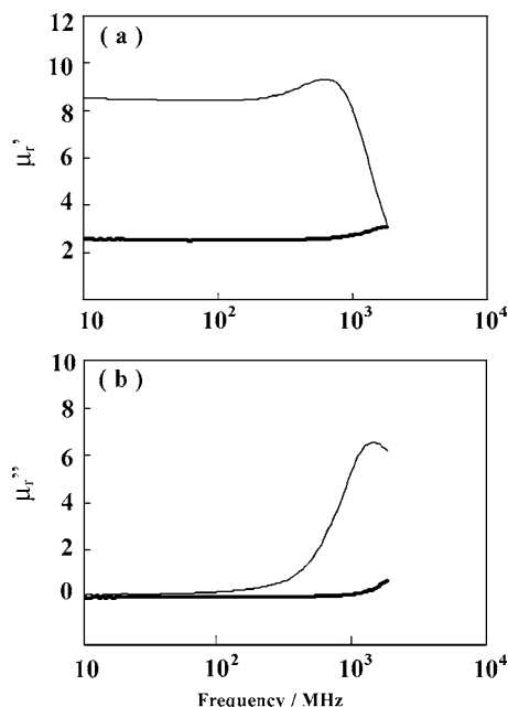
Figure 9 Variations in the (a) real and (b) imaginary parts of the initial permeability of the 0% glass added-specimen sintered at 1300°C for 1 h in air and the 5% glass added-specimen sintered at 1000°C for 1 h in air as the function of frequency. Thick lines are the 5% glass added-specimen and thin lines are the 0% glass added-specimen.
