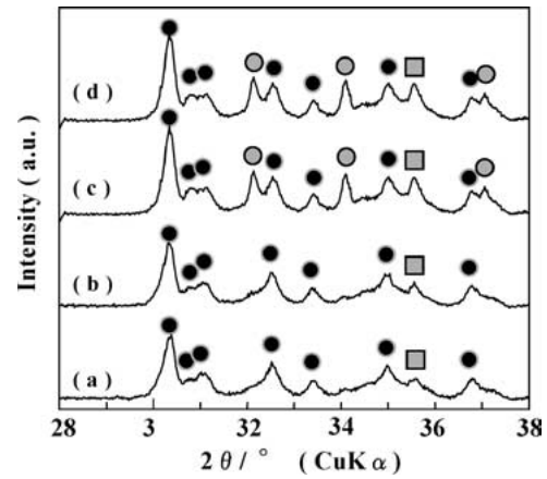
Figure 4 XRD patterns of the 5% glass added-specimen sintered at (a) 975°C for 1 h in air, (b) 1000°C for 1 h in air, (c) 1000°C for 10 h in the sealed platinum container and (d) at 1050°C for 1 h in air. (●): Co 2 Z, (○): Ba-M, (△): Co 2 W, (□): Spinel ferrite.
