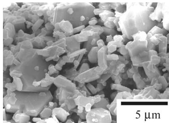
Figure 8 SEM photograph of the fractured surface of the 0% glass added-specimen sintered at 1000^\circ\text{C} for 10 h together with \text{MgF}_2 powder pellet in the sealed platinum container.
