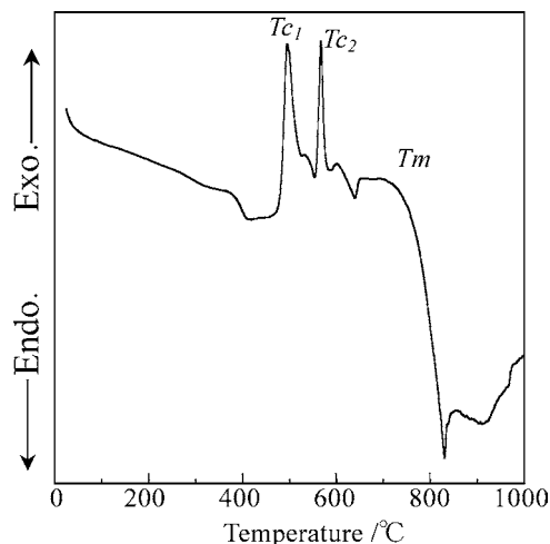
Figure 1 DTA curve of the additive glass.
