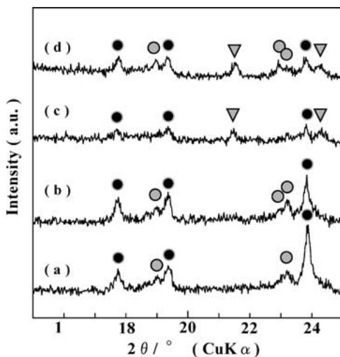
Figure 3 XRD patterns of the 0% glass added-specimen sintered at 1000°C (a) for 1 h in air and (b) for 10 h in the sealed platinum container and the 5% glass added-specimen sintered at 1000°C (c) for 1 h in air and (d) for 10 h in the sealed platinum container. (●): Co 2 Z, (○): Ba-M, (▽): Unknown.
