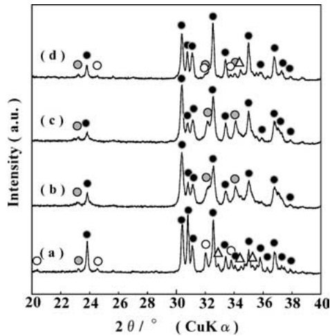
Figure 2 XRD patterns of (a) the as-calcined ferrite powder and the 0% glass added-specimen sintered at (b) 1000°C for 1 h in air, (c) 1000°C for 10 h in the sealed platinum container and (d) 1300°C for 1 h in air. (●): Co 2 Z, (○): Co 2 Y, (△): Co 2 W.
